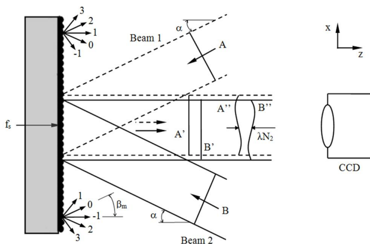
Fig. 1. Moiré interferometry principle [23].
