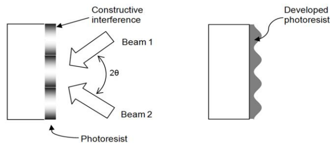
Fig. 2. Holographic grating obtained with photoresist [23].
