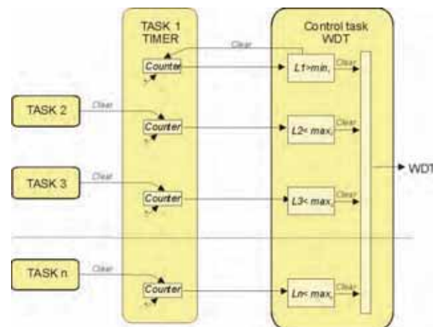
Fig. 4. Organization of the control task based on the call counters
