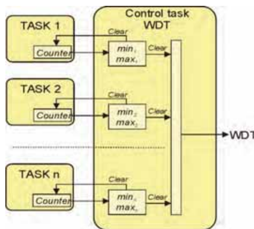
Fig. 5. Organization of the control task based on the measurements of the time between successive calls
