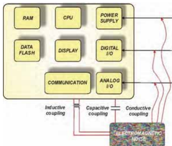
Fig. 1. Block diagram of a typical programmable device
