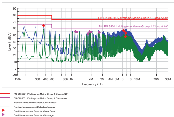
Fig. 3. Emitted electromagnetic disturbances (150 kHz – 35 MHz) measured on power supply lines of MPOF2
