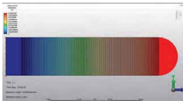
Fig. 7. Displacement as a function of applied voltage
