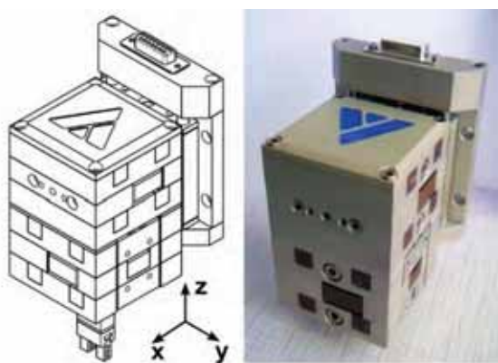
Fig. 5. CAD assembly of micropositioning system and mounted real device
