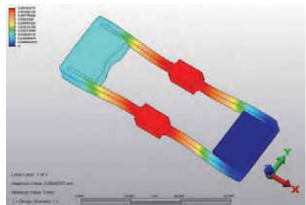
Fig. 9. Simulation screen of amplifier with load
