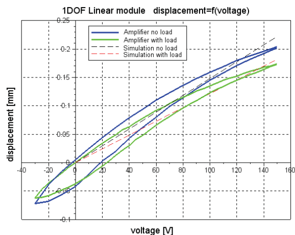
Fig. 13. Experimental and simulation test for mechanical amplifier and linear 1DOF module
