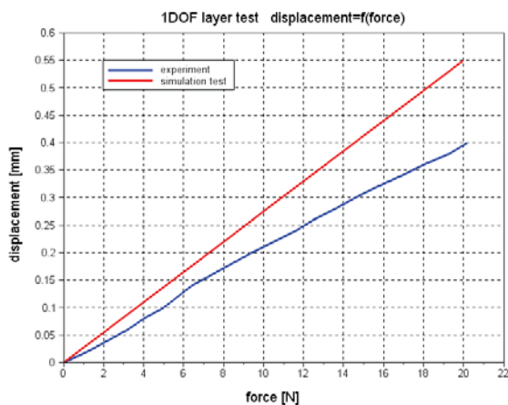
Fig. 12. Experimental and simulation test of 1DOF linear layer with 4 elastic hinges
