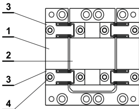
Fig. 2. A general concept of 1 DOF translational layer with flexure joints
