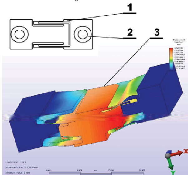
Fig. 8. Shape of 1 hinge and simulation results of a pair of flexure hinges
