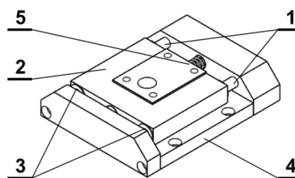
Fig. 4. General concept of linear Z movement system
