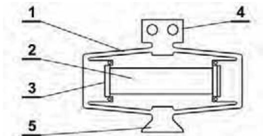
Fig. 3. Monolithic amplifier with mechanical slots (holes and dovetail) and piezoactuator mounted inside
