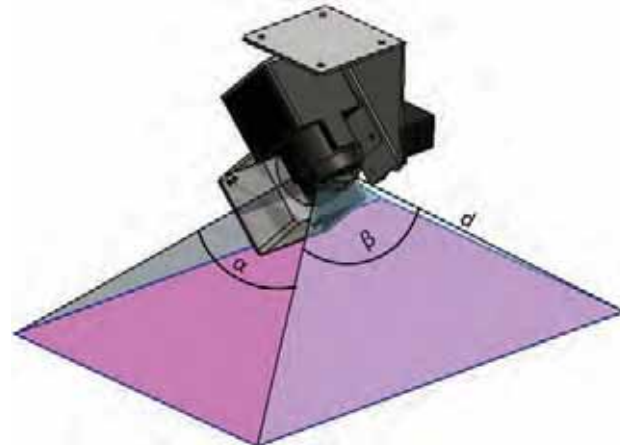
Fig. 3. Scanning coverage of the module
