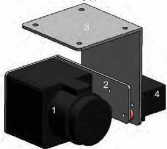
Fig. 1. Structure of the three-dimensional laser range scanner
