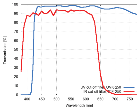
Fig. 4. The optical transmission of the VIS filters as a function of the wavelength
