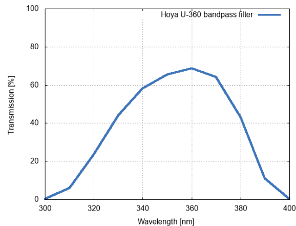
Fig. 3. The optical transmission of the NUV filter as a function of the wavelength
