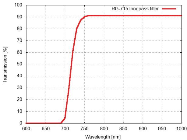
Fig. 5. The optical transmission of the NIR filter as a function of the wavelength
