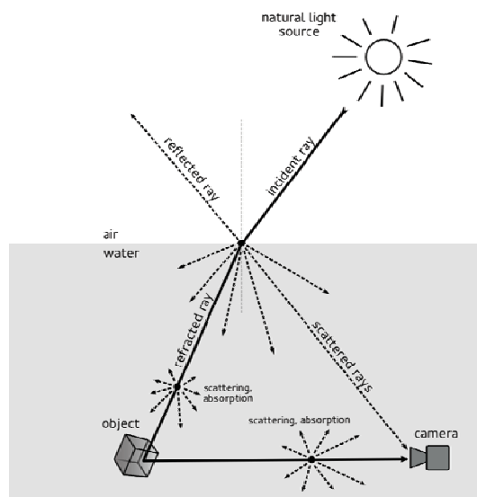
Fig. 2. The path of a single ray of the natural light reflected to the camera, letting to capture the image of that object
