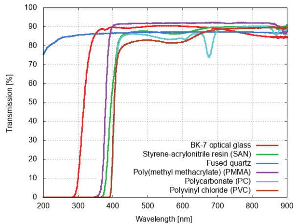
Fig. 7. The optical transmission of all tested transparent materials as a function of the wavelength
