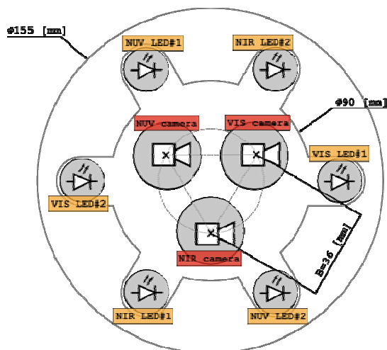
Fig. 6. The placement of elements (LEDs and cameras) of the TVS
