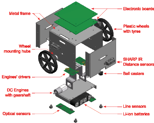
Fig. 2. SanBot mechanical structure overview
