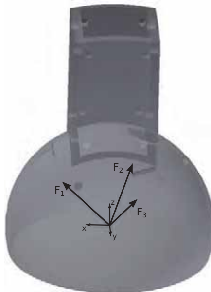
Fig. 7. Local coordinate frame for the foot. Forces F_1, F_2, F_3 point at each FSR
