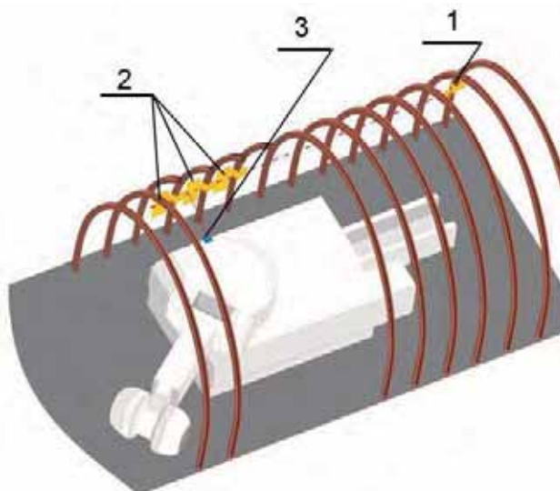
Fig. 11. Method of assembly of reflectors on ribs of the tunnel housing
