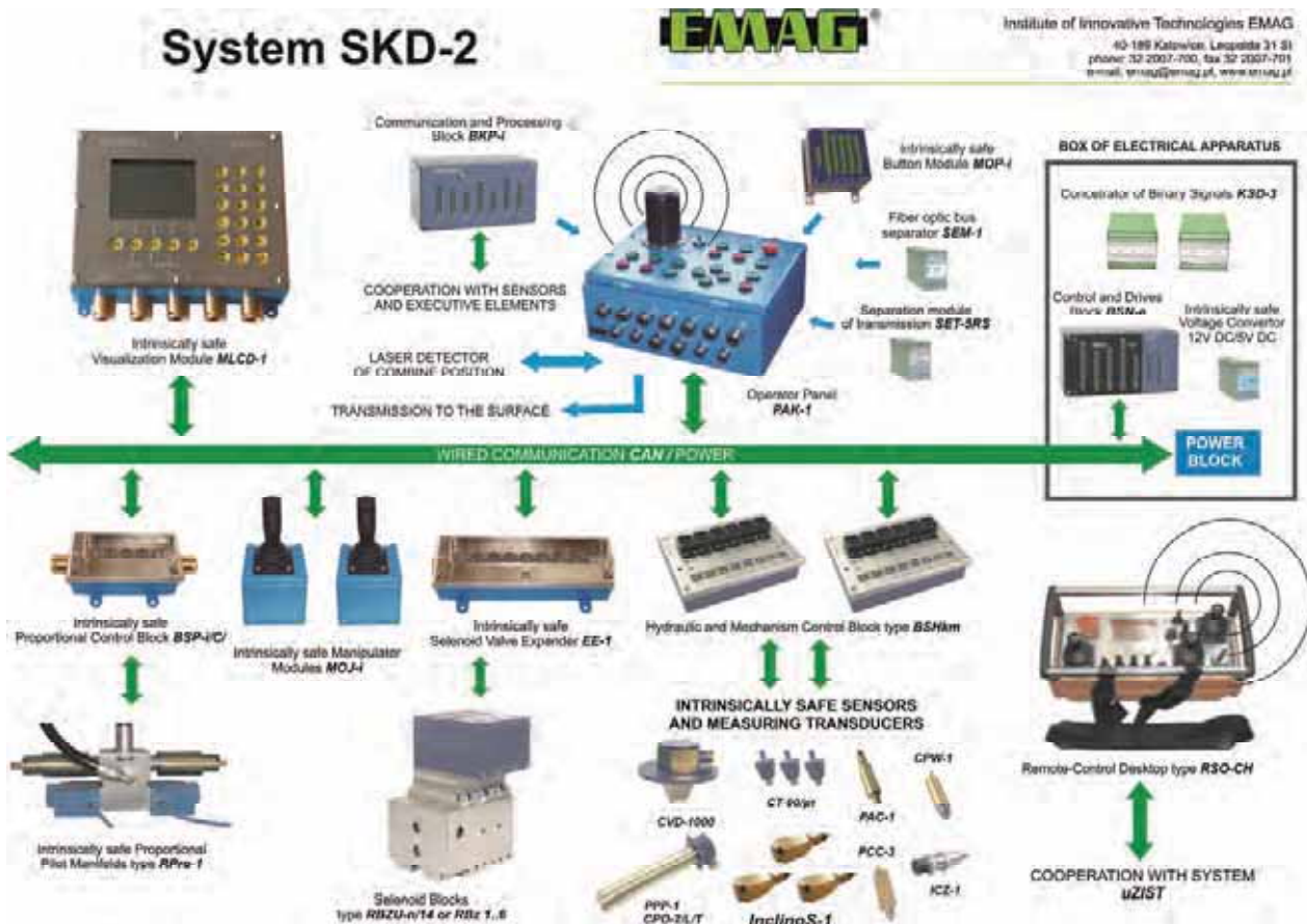
Fig. 2. SKD-2 system structure
