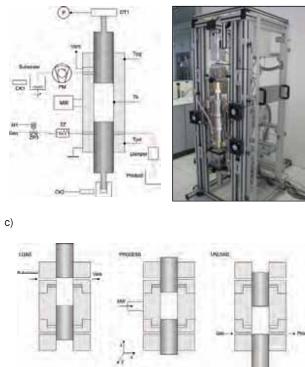
Fig. 1. General draft of the reactor (a), view of the prototype with the front cover taken off (b) principle of operation of the load and unload system (c)
