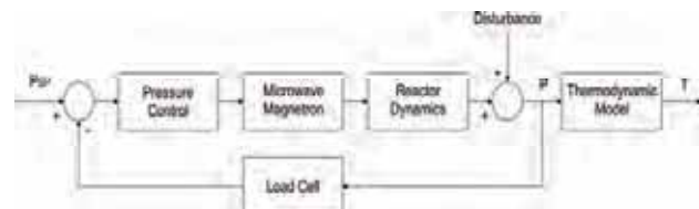
Fig. 3. Block diagram of pressure P regulation system and process temperature T determination
