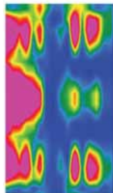
Fig. 2. Results of the analyses of the arrangement of the electromagnetic field for the MSS2 reactor: a) frequency characteristics for reflection coefficient |S_{11}| ; b) distribution of average bulk density of power losses in the xy plane; c) distribution of average bulk density of power losses in the xy plane; scale 5 \mu\text{W}/\text{mm}^2 , medium in the chamber – water
