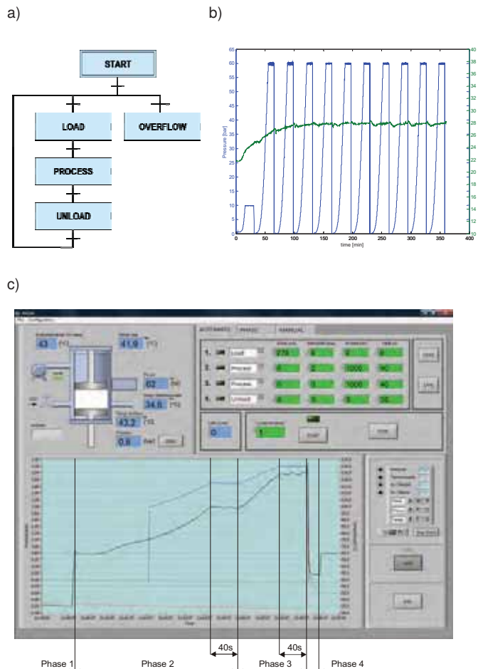
Fig. 5. Automatic (procedural) process control: a) process phases; b) course of process variables for cyclical recurrence of technological recipe realisation; c) image of the window of the control programme after realisation of a single recipe: Phase 1 – Load (278 ml), Phase 2 – Process (2 bar, 1 kW, 40s), Phase 3 – Process (3 bar, 1 kW, 40 s), Phase 4 – Unload (0, 20 s)
