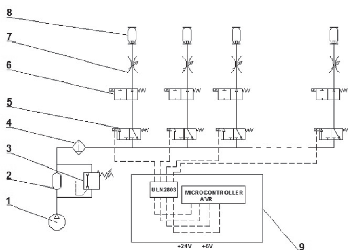
Fig. 10. Control system scheme: 1 – air compressor, 2 – compressed air tank, 3 – pressure valve, 4 – air filter, 5 – reversing 3/2 valves, 6 – cut-off 2/2 valves, 7 – throttle valves, 8 – McKibben-type muscles, 9 – electronics
