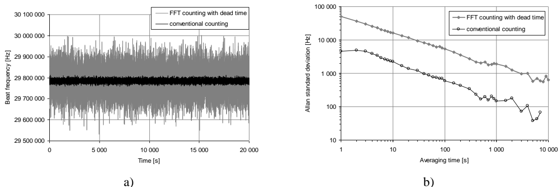
Fig. 4. a) Example of frequency counting of the beat between a iodine frequency stabilized He-Ne laser and fs-comb. b) Corresponding Allan standard deviation.
