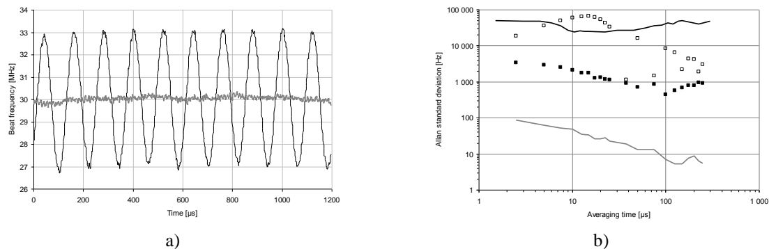
Fig. 7. a) Black line shows frequency modulation of the beat between fs-comb and He-Ne laser and the grey line shows residuals after subtraction of modulation (i.e. stability of carrier frequency). b) Corresponding Allan standard deviation (black line) of carrier frequency (for a single 1.2 ms interval) compared to FFT counting capability for 10 MHz signal of reference frequency (grey line). The Allan standard deviation for a beat frequency between two He-Ne lasers is plotted for comparison – with unwanted frequency modulation (open squares) and after its subtraction (filled squares).
