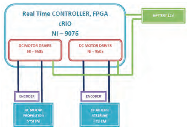
Fig. 18. Mobile platform electrical scheme
