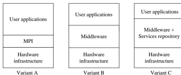
Fig. 1. Alternatives to development of applications for cluster-oriented environment.
