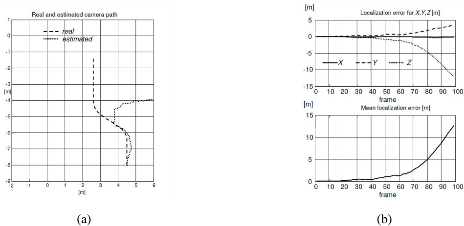
Fig. 7. Comparison of real and estimated path of the stereovision module a) and localization errors b) for a purely vision-based egomotion algorithm.
