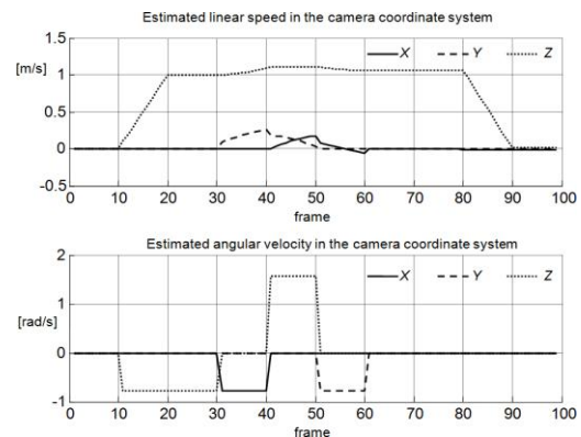
Fig. 5. Plots of estimated motion parameters as a function of frame number.
