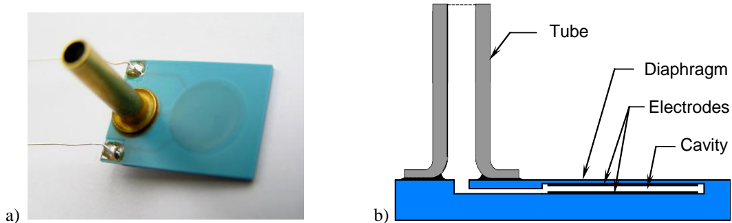
Fig. 1. Capacitive CPS in LTCC structure: a) the prototype and b) the schematic representation of the cross-section (not to scale).
