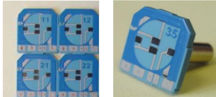
Fig. 3. Prototypes of the LTCC-based piezoresistive CPS.
