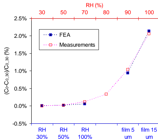
Fig. 2. Measured and simulated changes in C_0 for different situations. (The bottom X-axis is for FEA assumptions and the top X-axis is for the measurement results).
