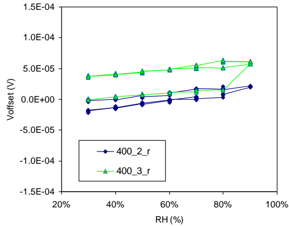
Fig. 6. Offset voltage versus relative humidity for the sensors with 400- \mu m diaphragm after two additional RH cycles.
