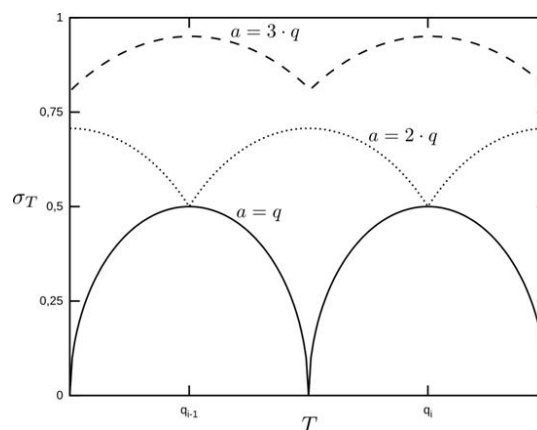
Fig 10. Characteristics of standard deviation of a measurement series for different widths of rectangular distribution.
