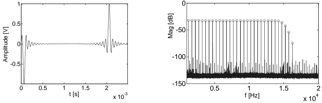
Fig. 13. The time plot of the SINC signal - 31 Tones, CF = 7.8 , BW = 15 kHz.
