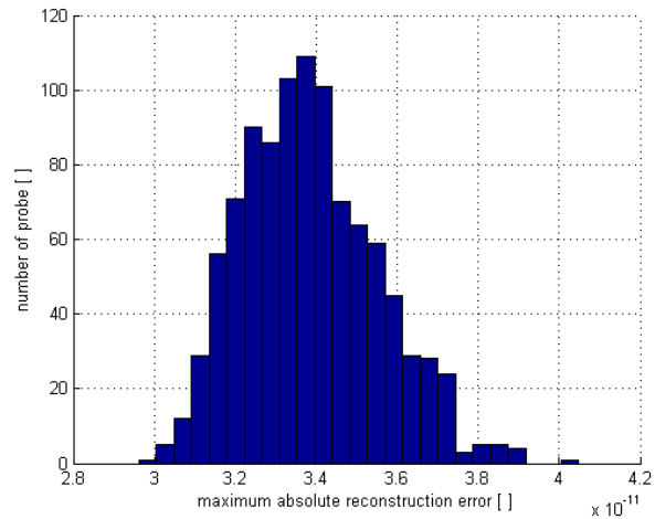
Fig. 13. Histograms of maximum absolute reconstruction error for a test signal with random phases (values from the uniform distribution in the interval [0^\circ, 360^\circ] ). Left – signal with normal white noise ( SNR=90 dB), right – signal without noise. Matrix F without error.
