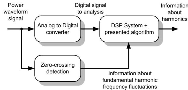
Fig. 14. Variable-frequency least squares Prony method – example of its application in an electrical power quality monitoring system.
