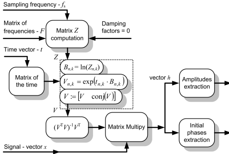
Fig. 1. Variable-frequency reduced least squares Prony method.
