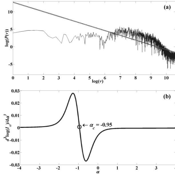
Fig. 3. (a) Log-log plot of PSD P_H(v) versus frequency v - (b) Third order derivative of the logarithmic function and the zero crossing point - of the WF movement from electrode position 1 of subject 1. Note that in (a), the solid line is P_H(v) and the diagonal dash line is the slope of the log-log plot of the P_H(v) , which is estimated by linear regression.
