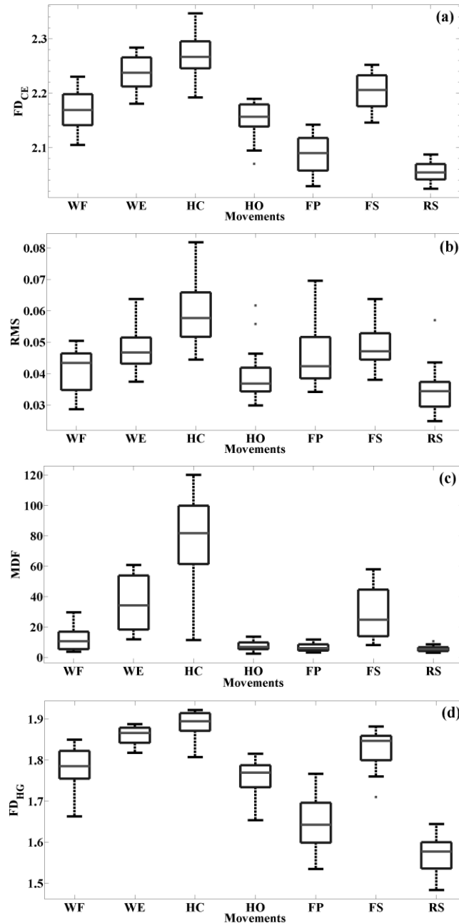
Fig. 5. Box plot of (a) FD_{CE} (b) RMS (c) MDF (d) FD_{HG} from 7 hand movements of the subject 27 and electrode position 1.
