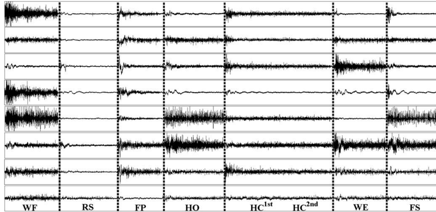
Fig. 4. Graphical representation of the eight-channel sEMG signals according to the seven hand movements.
