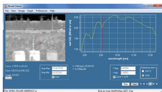
Fig. 12. The results of freon 134 measurements (concentration 3%, distance 60 m, T_{atm} = 18^{\circ}C , v_{wind} = 8 m/s , p_{atm} = 992 hPa): (a) spectral characteristics, (b) results of analysis in Matlab.
