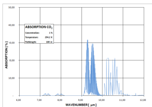
Fig. 7. The absorption of selected gases: (a) CO 2 (concentration 1%), (b) NO 2 (concentration 1%).
