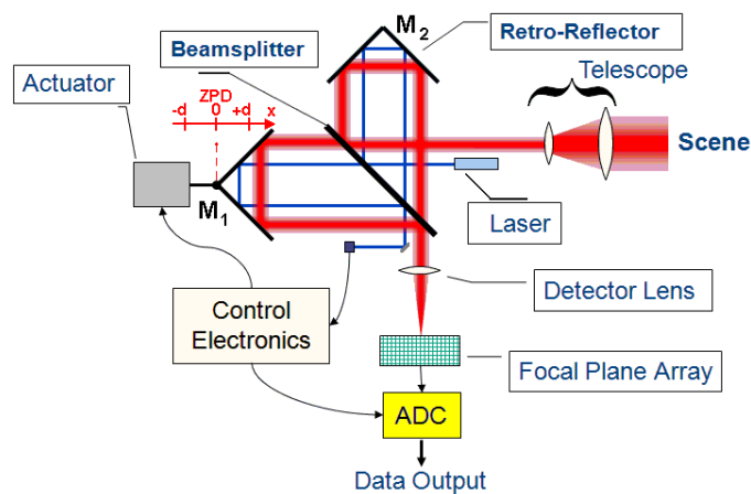
Fig. 4. Block diagram of imaging Fourier-transform spectroradiometer.
