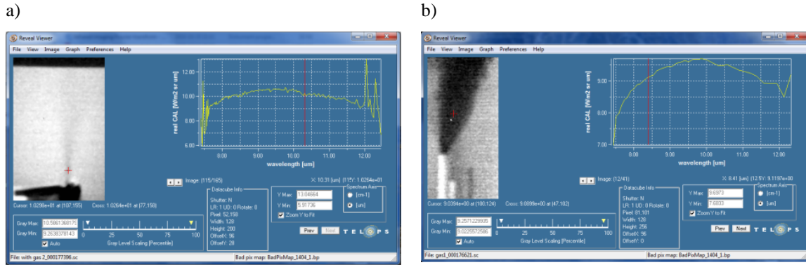
Fig. 8. The spectral results of gas measurements during laboratory tests: (a) CO 2 (concentration 1%, ΔT= 1 K), (b) NO 2 (concentration 1%, ΔT=3 K).
