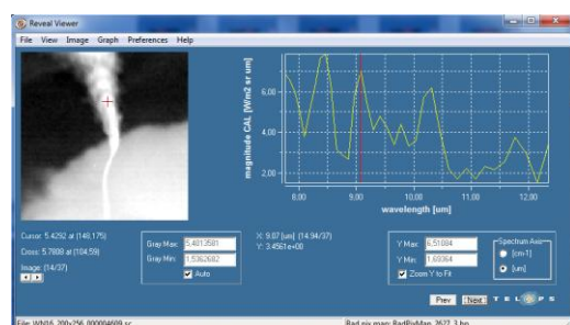
Fig. 12. The results of freon 134 measurements (concentration 6%, distance 10 m, T_{atm} = 21^{\circ}C , v_{wind} = 1 m/s , p_{atm} = 998 hPa) : (a) spectral characteristics, (b) results of analysis in Matlab.
