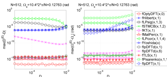
Fig. 4. Systematic errors of damping and frequency estimation as a function of damping.
