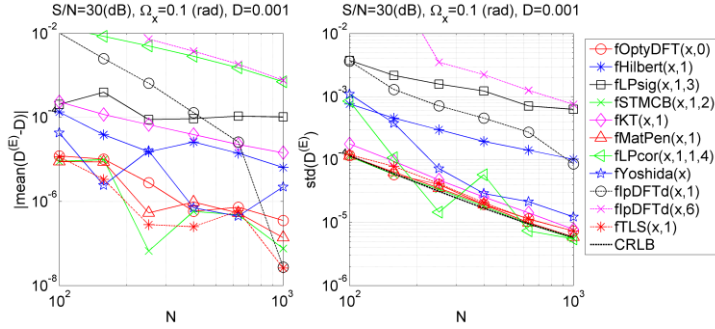
Fig. 9. Mean value and standard deviation of damping estimation.
