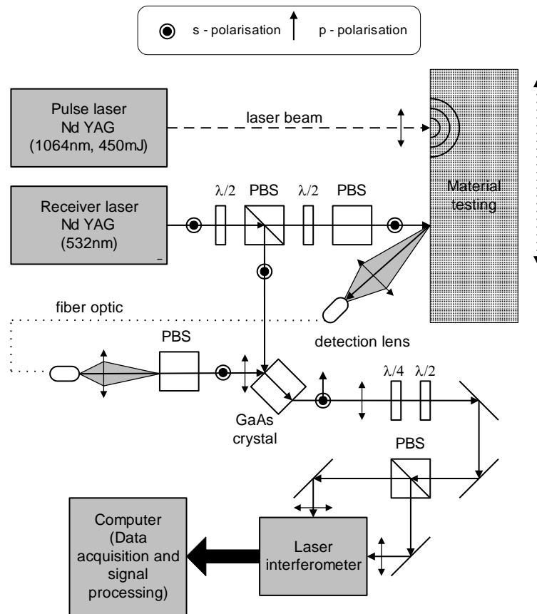
Fig. 5. Laser ultrasonic set-up.
