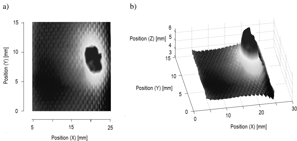
Fig. 7. Example C-scan (20x15 \mu\text{m} ) of 35 J impact damage on the material: a) 2-D, b) 3-D.
