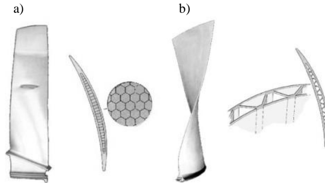
Fig. 2. Examples of blade constructions with armour: a) honeycomb, b) openwork construction.
