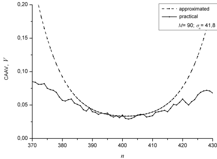
Fig. 1. The characteristics of conditional averaging of absolute value of the delayed signal surrounding its minimum.
