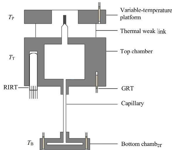
Fig. 1. Sealed-cell for the realization experiment.
