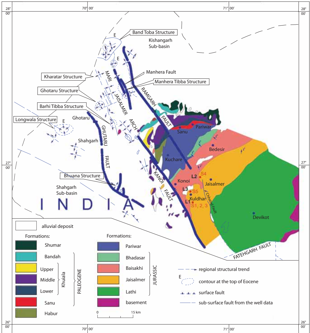
Fig. 2. Geological map of the Jaisalmer Basin (after Das Gupta, 1975) showing localities L1, L2, L3 and the location of sections (S1–S5) investigated in the present study
