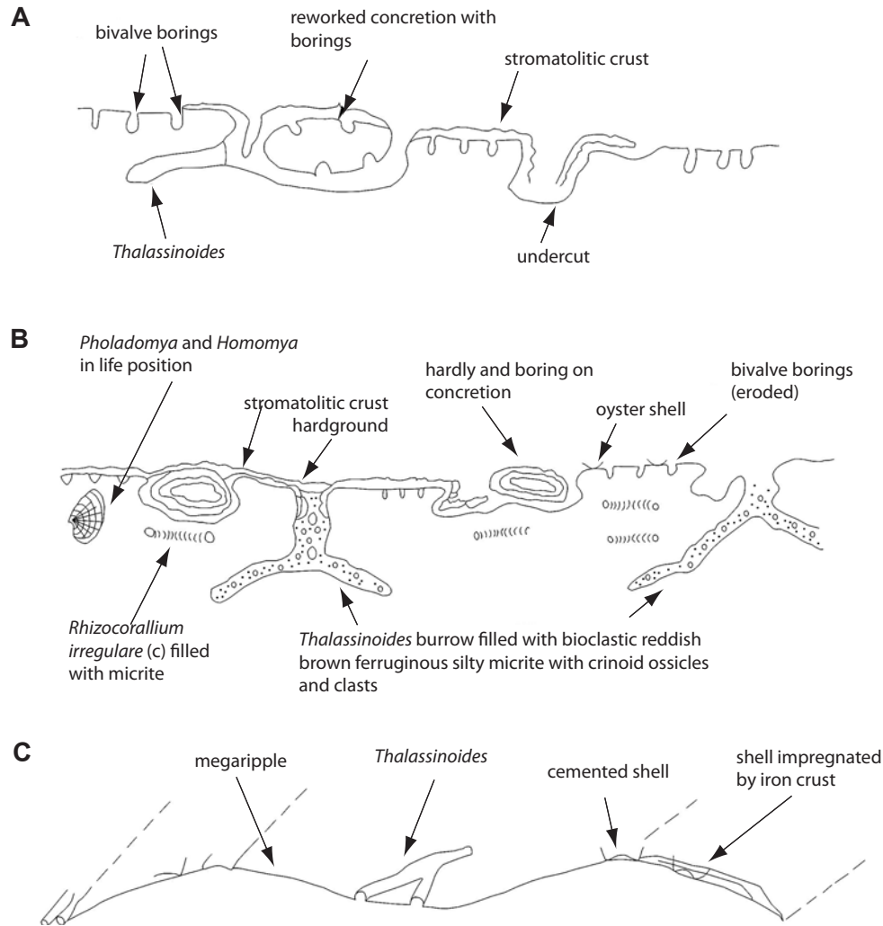
Fig. 5. Sketch diagram of hardground surfaces I, II and III in the Kuldhar Member at Kuldhar River-section (S1 in Fig. 3), south of the Kuldhar Village in the east of the Kuldhar River (locality L1 in Fig. 2), 16 km southwest of Jaisalmer City (Fürsich et al. , 1992)
