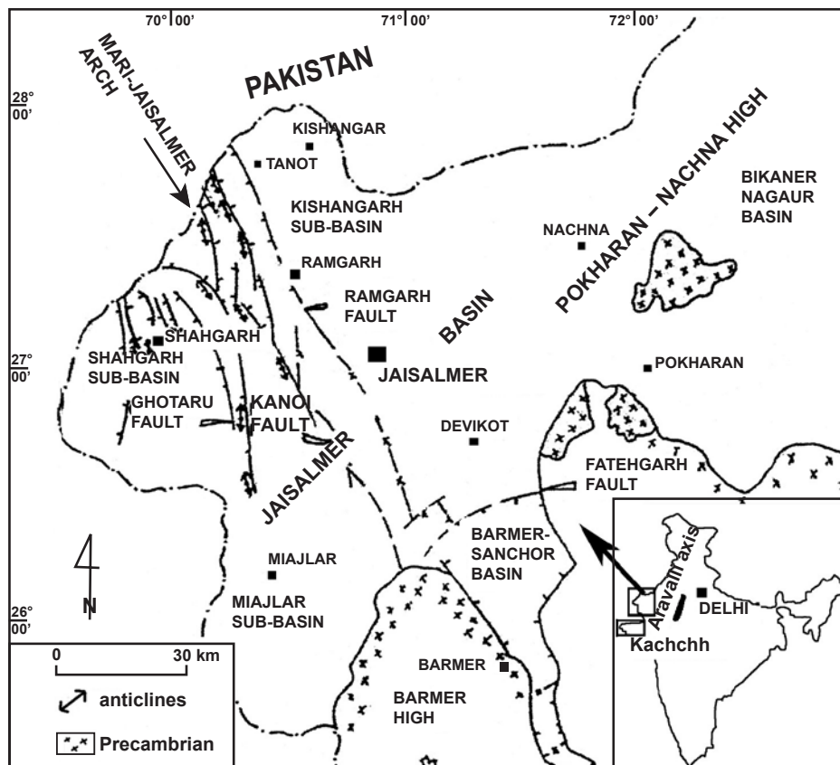
Fig. 1. Location map. Structural elements in western Rajasthan (modified after Misra et al. , 1993)
