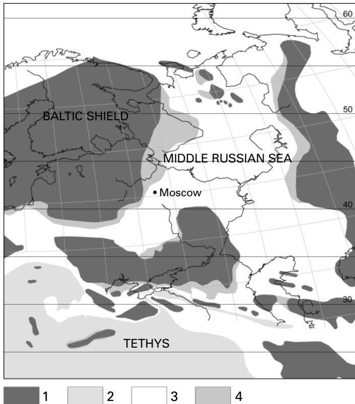
Fig. 1. Middle Russian Sea and adjacent areas during the Late Jurassic (example of Late Kimmeridgian – Early Volgian): 1 – land areas; 2 – oceanic basins; 3 – shallow epicontinental seas; 4 – coastal areas, sometimes flooded by sea. Palaeogeography and paleolatitudes are from Thierry and Barrier (2000), corrected.
