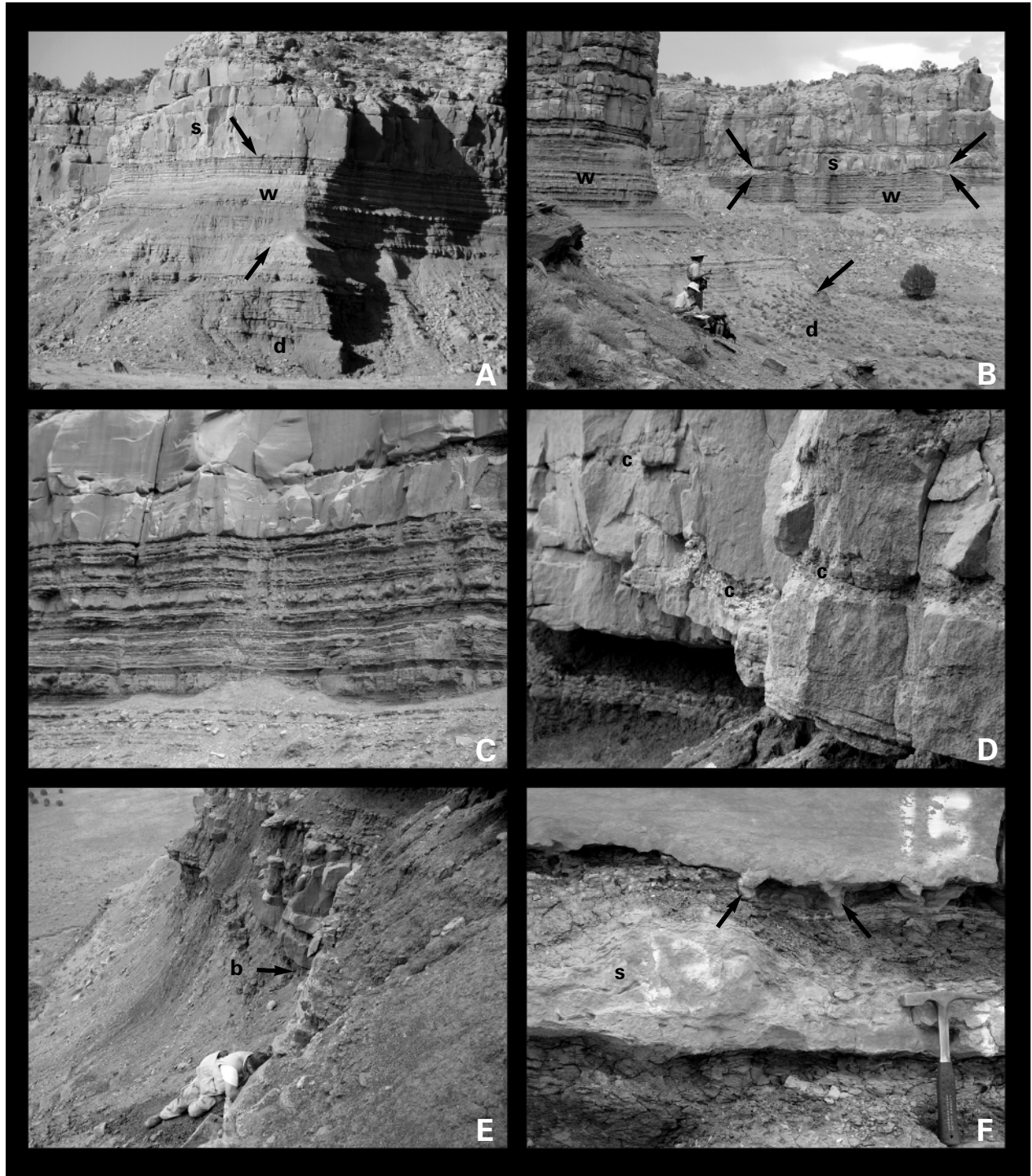
Fig. 4. A – Outcrop at Whitmore Point, the type location for the Whitmore Point Member. Arrows at the contact between Dinosaur Canyon Member (d) and Whitmore Point Member (w) and at upper contact of Whitmore Point strata with the Springdale Sandstone Member of the Kayenta Formation (s). B – Overview of the Whitmore Point Member 2 km to the west of the type locality. Arrows at lower Whitmore Point (w) contact and at contact with overlying “Dinosaur Canyon” type sandstones. Springdale Sandstone (s) above scours down into these sandstones. C – Highlight from location B illustrating lateral continuity of interbedded shales, siltstones and sandstones. D – Contact of fine-grained Whitmore Point strata and coarse-grained Springdale sandstones with conglomeratic lenses (c). E – Slope of Unit 3 (at location B) exposing gray and black shale. A black shale bed (b) underlies the sandstone ledge. F – Limestone bed at base of Whitmore Point section at St. George, Utah (Johnson Farm track site) contains a domal stromatolite (s). The sandstone layer above (labeled 15) hosts a tetrapod trackway on the upper surface. Sandstone-filled desiccation cracks (arrows) extend downward from the base of the sandstone bed.
