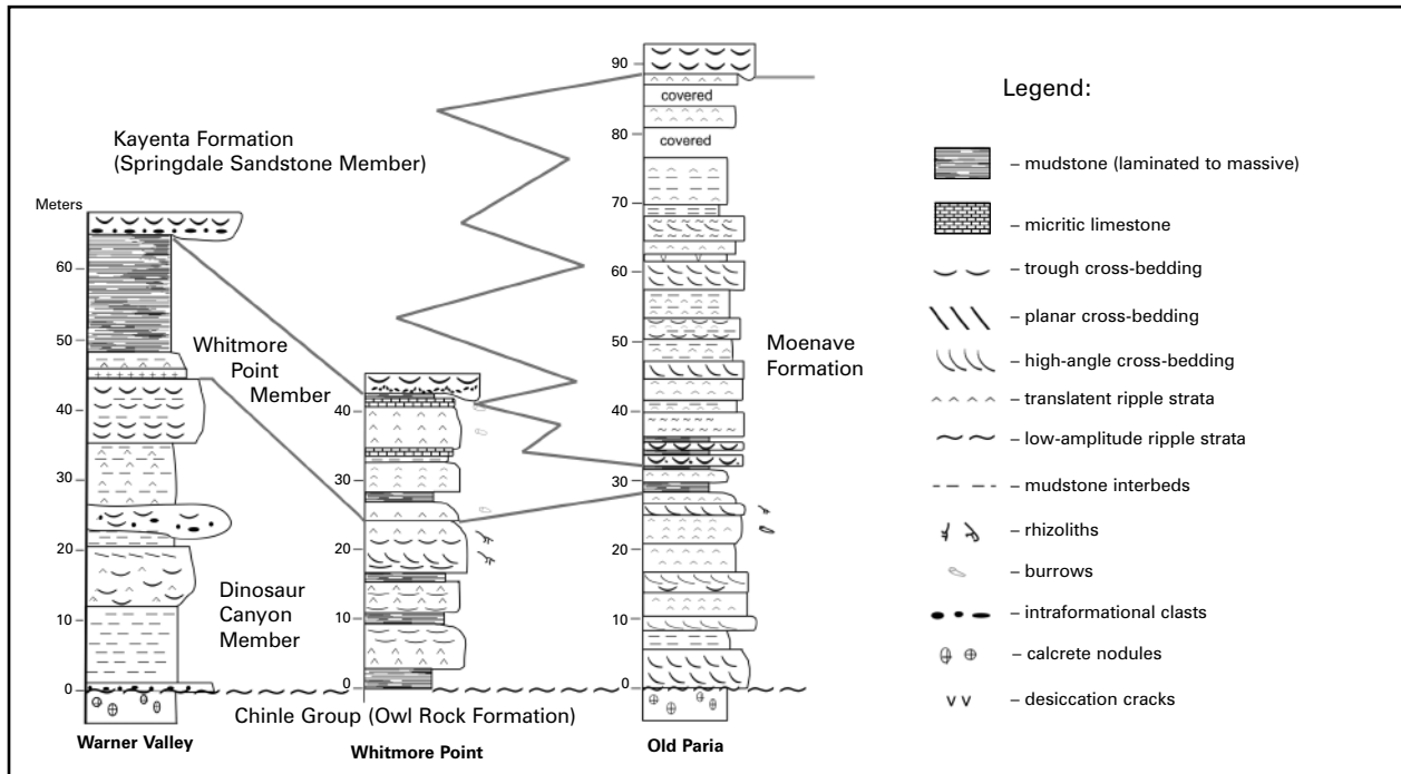
Fig. 3. Cross-sections illustrating lateral relationships of lithofacies for the Moenave Formation. West-east cross-section across northern part of study area from Warner Valley (near St. George) to Old Paria. No horizontal scale is implied (see Fig. 1 for section locations).
