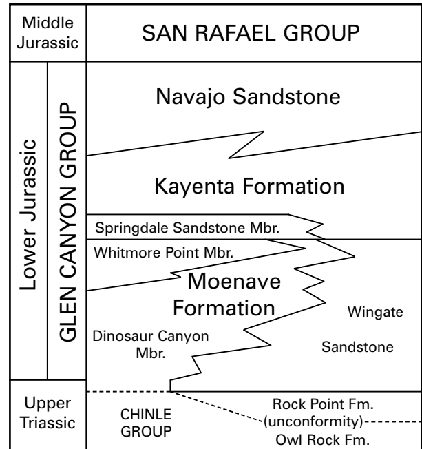
Fig. 2. Stratigraphy of Upper Triassic and Lower Jurassic in the study area.
