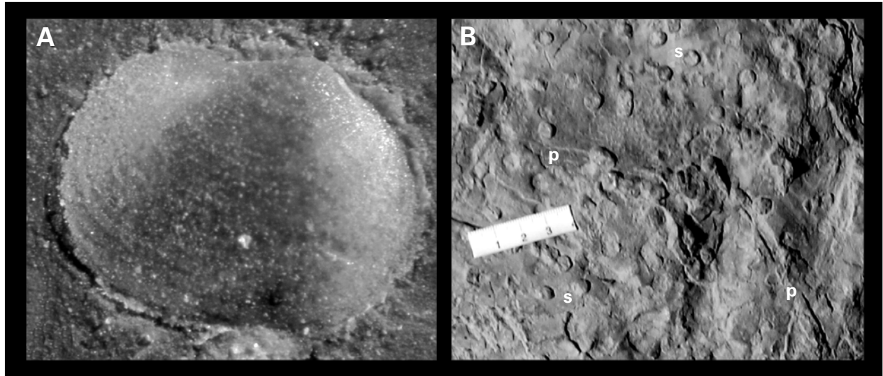
Fig. 5. Selected fossils from the Whitmore Point Member of the Moenave Formation (all from Johnson Farm, St. George, Utah): A – right valve of the conchostracan Euestheria ; valve is about 3.5 mm wide; B – Skolithos (s) and Palaeophycus ichnosp. (p) burrows on sandstone surface characteristic of ichnofossil assemblage of the Scoyenia ichnofacies (scale bar in cm).
