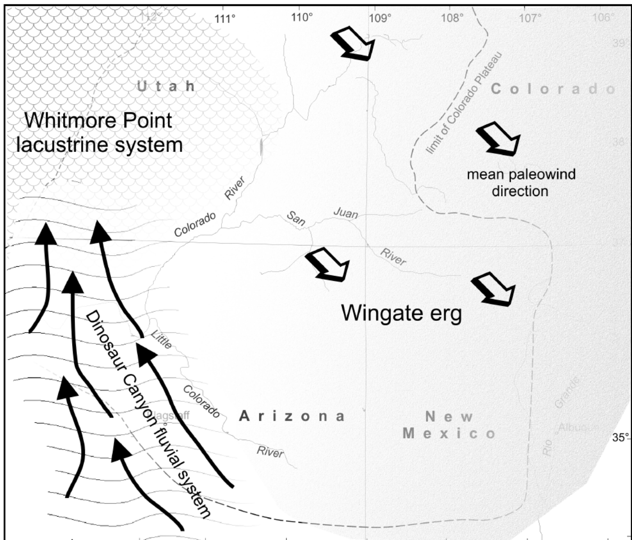
Fig. 6. Paleoenvironmental reconstruction for the Colorado Plateau area during Early Jurassic deposition of the Moenave Formation and Wingate Sandstone.
