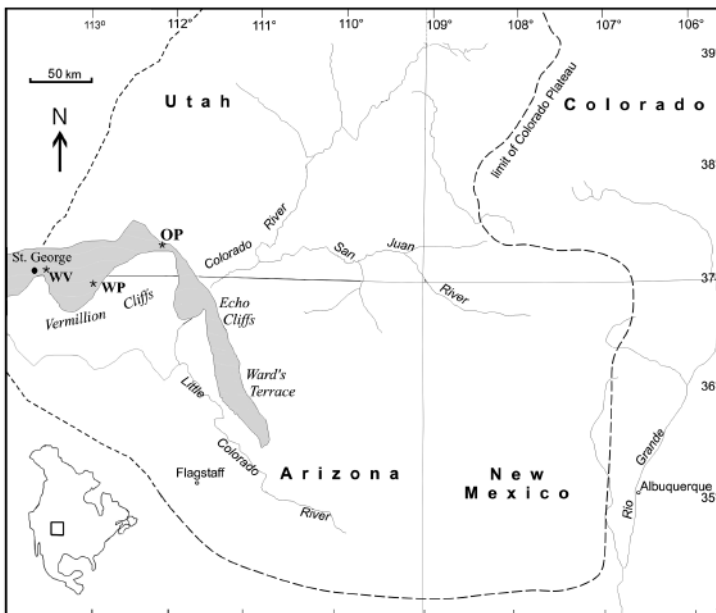
Fig. 1. Location map outlining the position of the Colorado Plateau and area of outcrop of the Moenave Formation (shaded gray), including the Dinosaur Canyon and Whitmore Point members. Old Paria (=OP), Whitmore Point (=WP) and Warner Valley (=WV) are locations referred to in text at which sections in Fig. 3 were measured.
