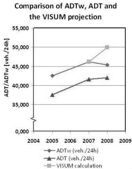
Fig. 9. Visualisation of the average daily traffic (ADT = all days, ADTw = working days), see comment in Table 1
