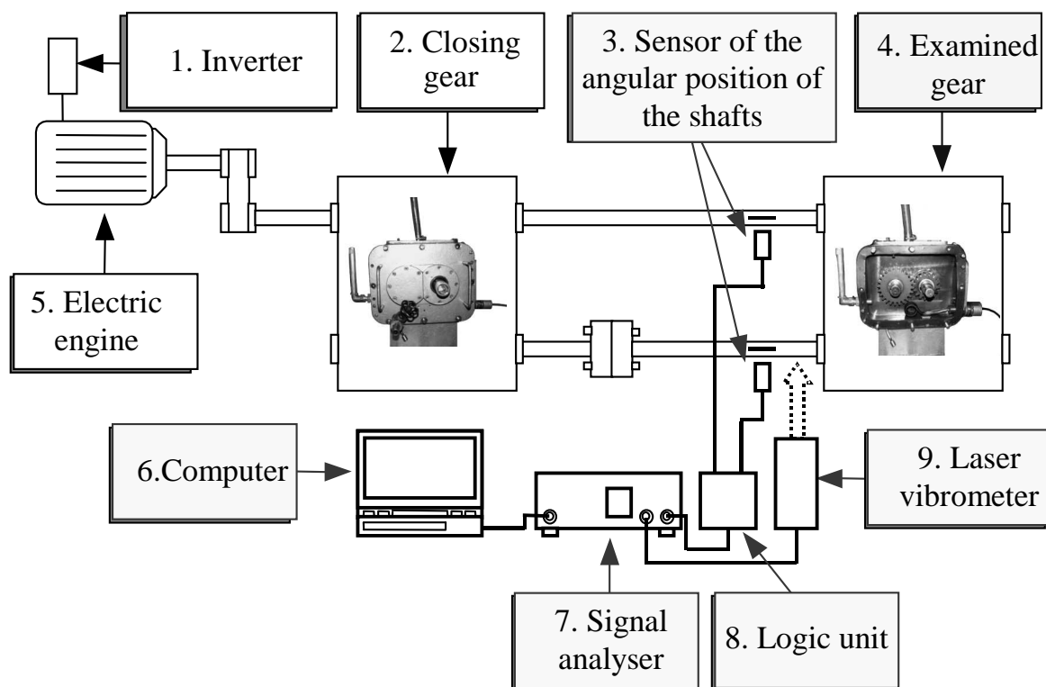
Fig. 2. Scheme for the measuring system (1-inverter, 2-closing gear, 3-sensor of the angular position of the shafts, 4- the examined gear, 5- electric engine, 6-computer, 7- the signal analyser, 8- logic unit, 9- laser vibrometer)
