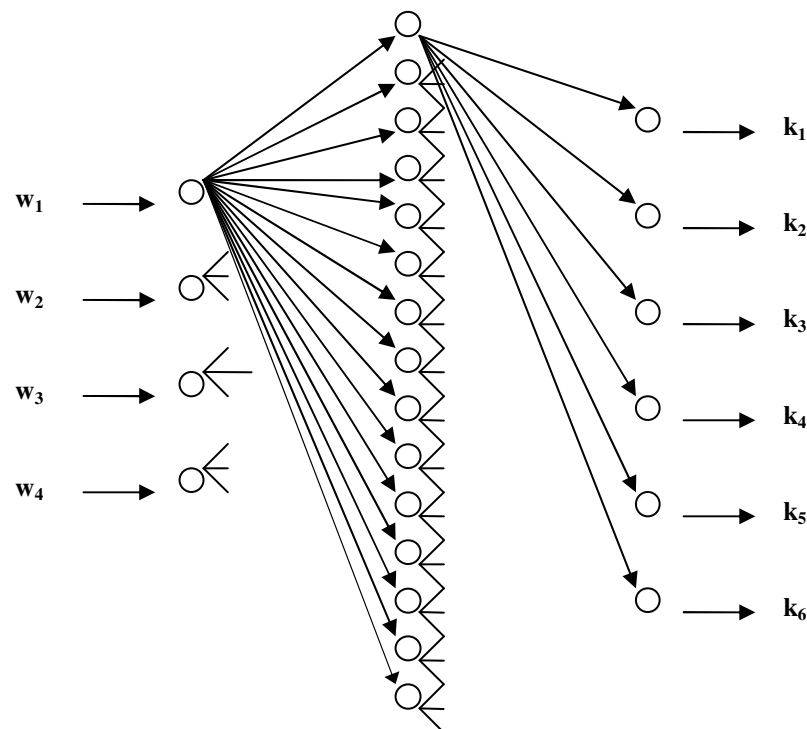
Fig. 5. Structure of the neural network
