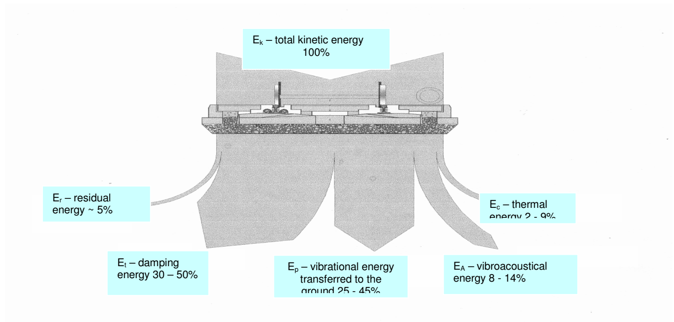
Fig. 9. Energetic balance of vibroisolated railway crossing
