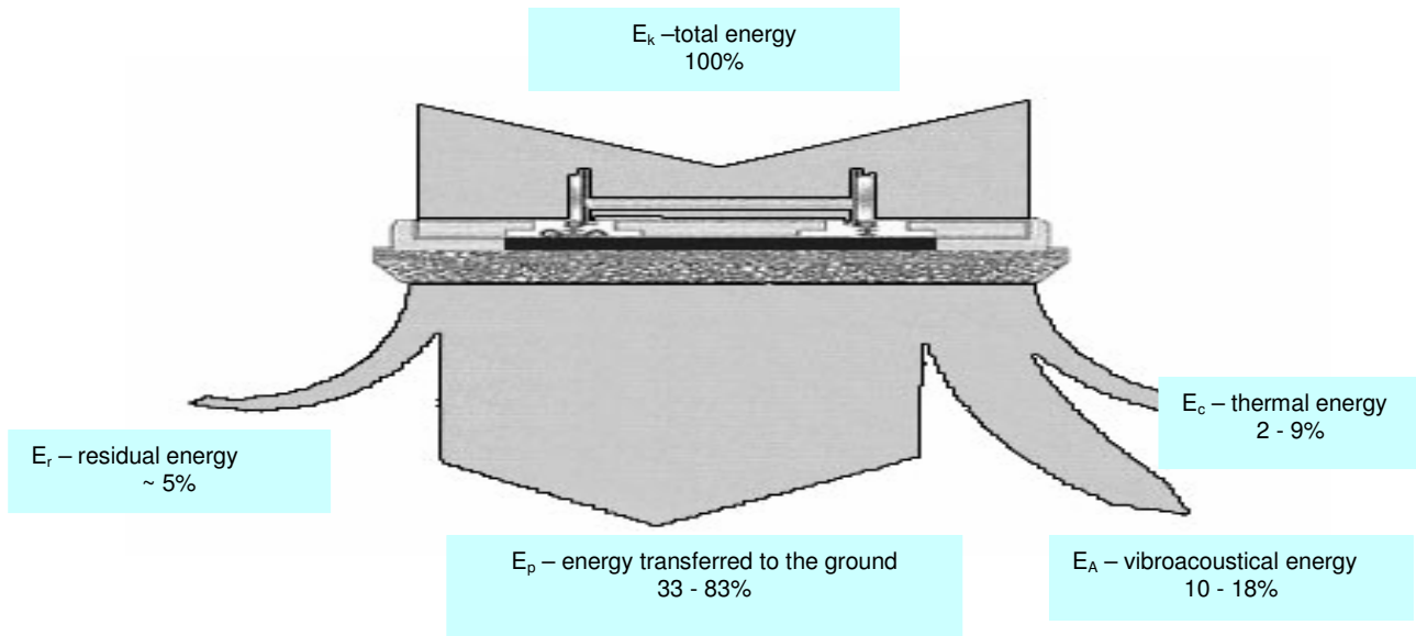
Fig. 10. Energetic balance of traditional railway crossing
