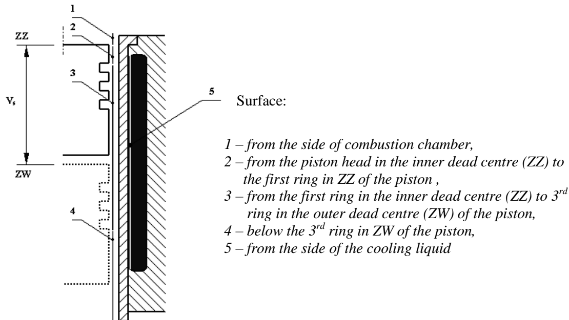
Fig. 1. The wet cylinder sleeve Rys. 1. Mokra tuleja cylindra
