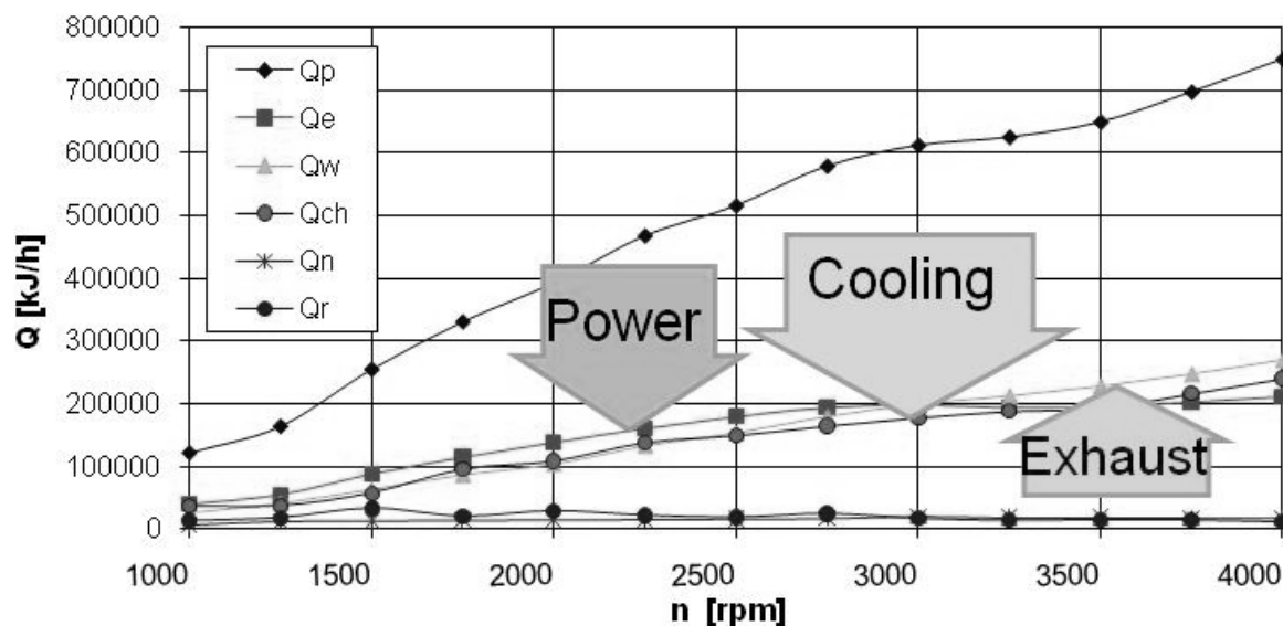
Fig. 1. Comparison of heat engine 4CT90 streams (designation: Q_p – heat from the combustion of fuel spilled, Q_e – heat converted into useful work, Q_{ch} – dissipate heat to the cooling system, Q_w – convection heat from the exhaust gases, Q_r – the rest of the balance, and the heat discharged into the environment from the hot walls of the engine and other losses)
