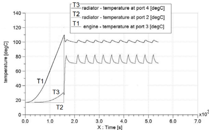
Fig. 3. Course characteristics at the pressure of 0,15 MPa and 96% of the filling with coolant: a) pressure: P1 – small circuit, P2 – large circuit, b) temperature: T1 – out of the cylinder block, T2 – entrance to the radiator, T3 – out of the radiator
