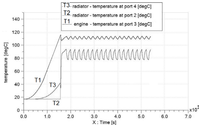
Fig. 4. Courses characteristics at the pressure of 0,15 MPa and 81% of the filling with coolant: a) temperature: T1 – out of the cylinder block, T2 – entrance to the radiator, T3 – out of the radiator
