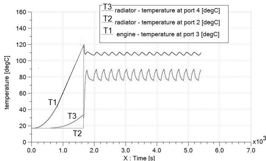
Fig. 5. Course characteristics at the pressure of 0,2 MPa and 96% of the filling with coolant : a) pressure: P1 – small circuit, P2 – large circuit, a) temperature: T1 – out of the cylinder block, T2 – entrance to the radiator, T3 – out of the radiator
