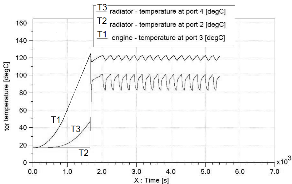
Fig. 6. Courses characteristics at the pressure of 0,2 MPa and 81% of the filling with coolant: temperature: T1 – out of the cylinder block, T2 – entrance to the radiator, T3 – out of the radiator
