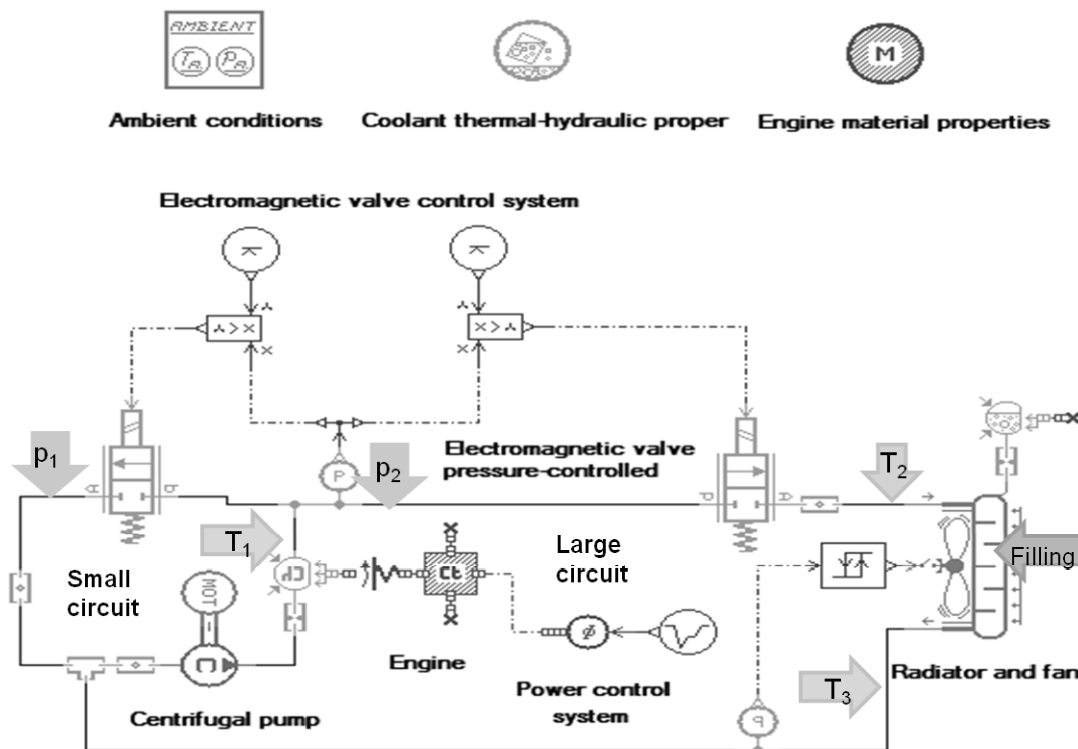
Fig. 2. Model stand scheme of cooling system developed in AMESIM software
