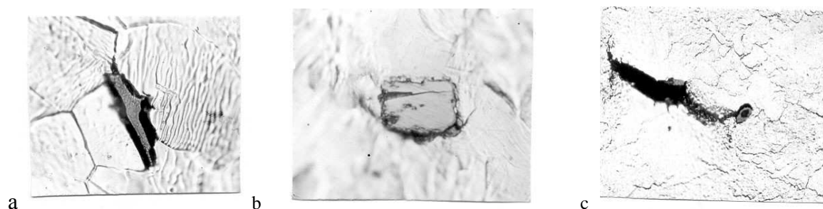
Fig. 1. Microbreaks near nonmetallic inclusions after plastic deformation; x600
