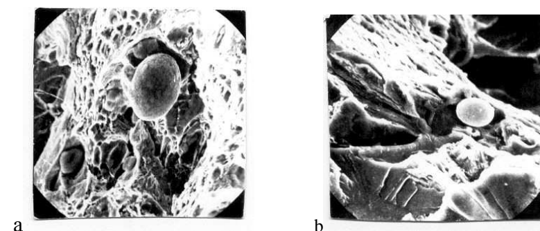
Fig 2. Fractures of wheel steel with nonmetallic inclusions; x2000
