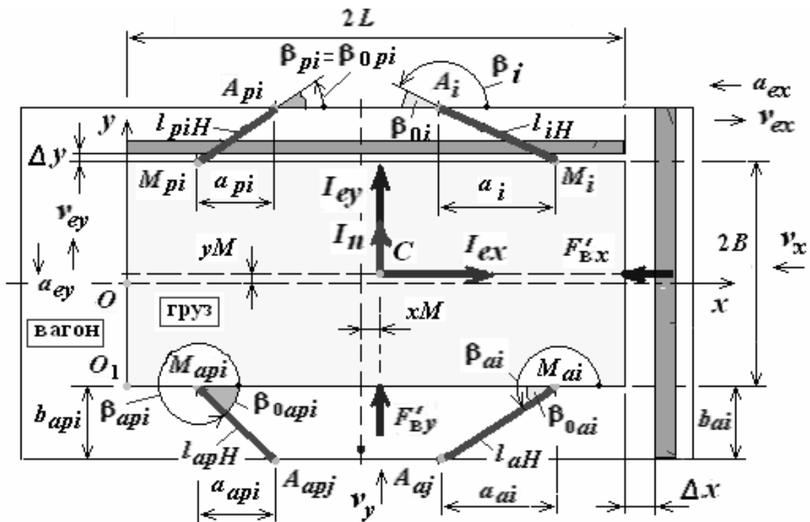
Fig. 1b. Physical modeling allocation cargoes in wagon, running on the curve section of railway descent (top view)
