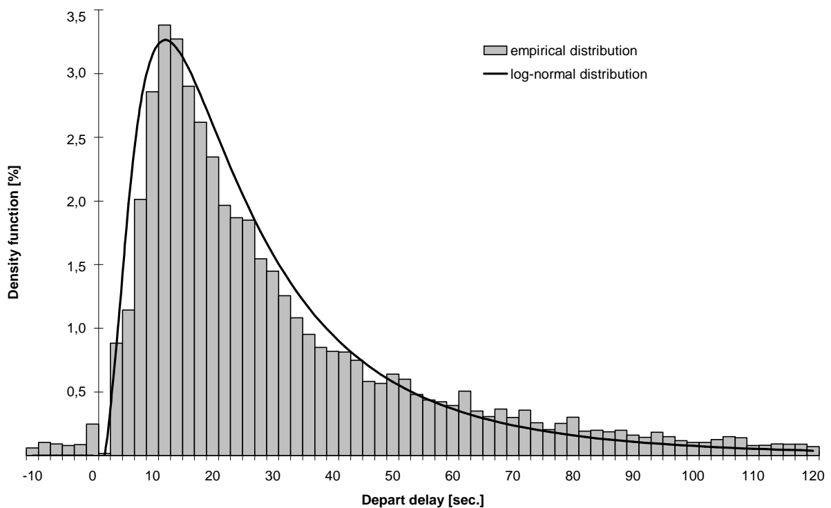
Fig. 3. Empirical density function for respective delay value and approximate to it log-normal distribution
