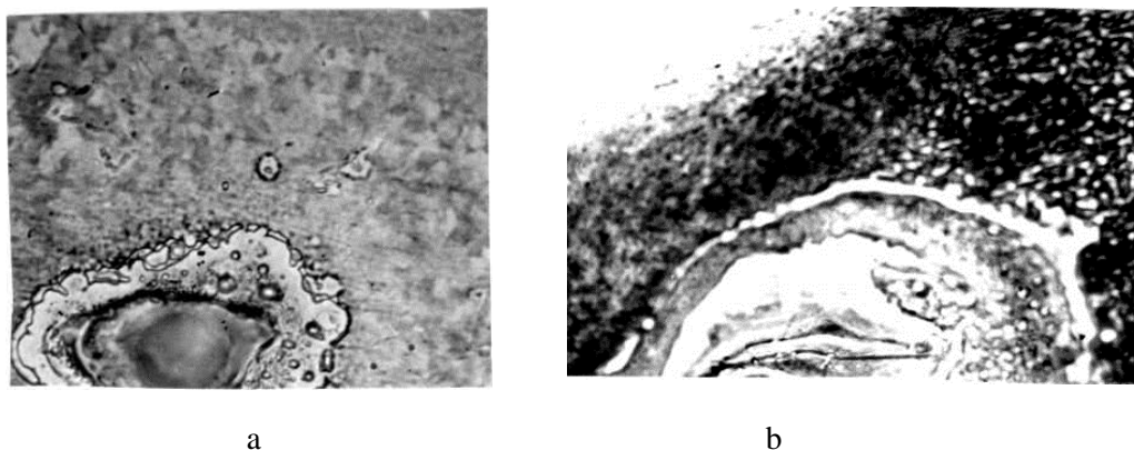
Fig. 3. Zones of local strengthening near non-metallic inclusions of oxide (a) and sulphide, (b) after laser treatment; \times 500
