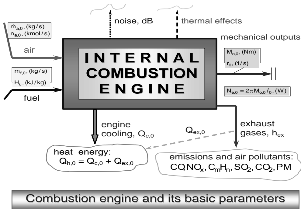
Fig. 2. Internal combustion engine as a complex energy object
