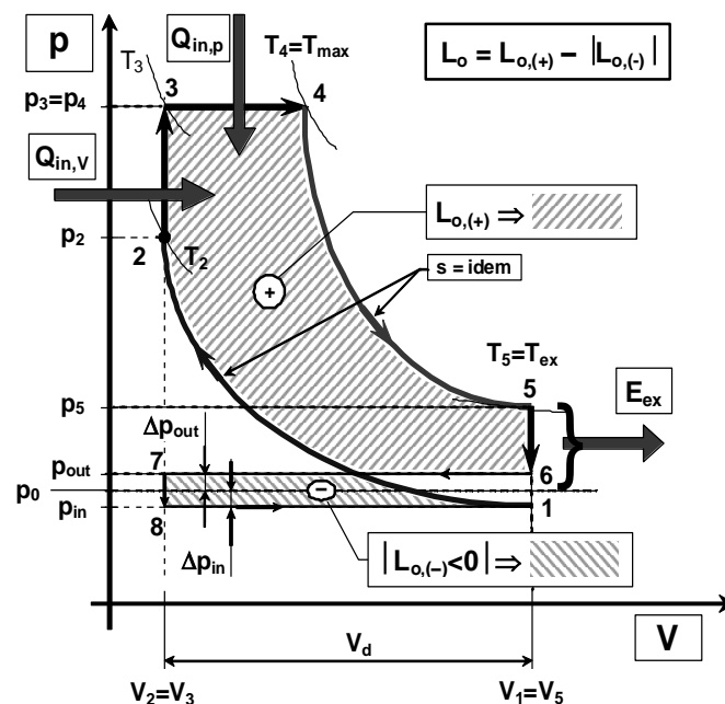
Fig. 6. Typical reference (Seiliger-Sabathe) cycle of IC engine accounting to the charge exchange work
