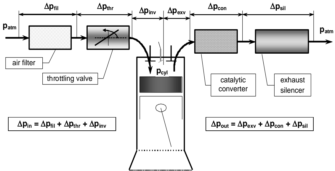
Fig. 4. Main elements of the charge exchange system (throttle valve for IC spark ignition engine)
