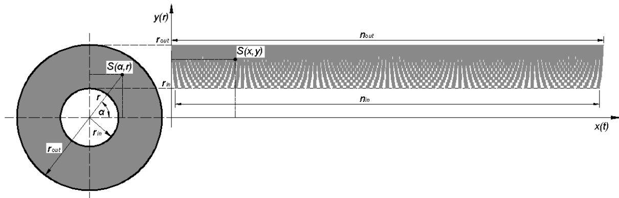
Fig. 1. Schematic diagram: circular disc and disc converted to rectangular form
