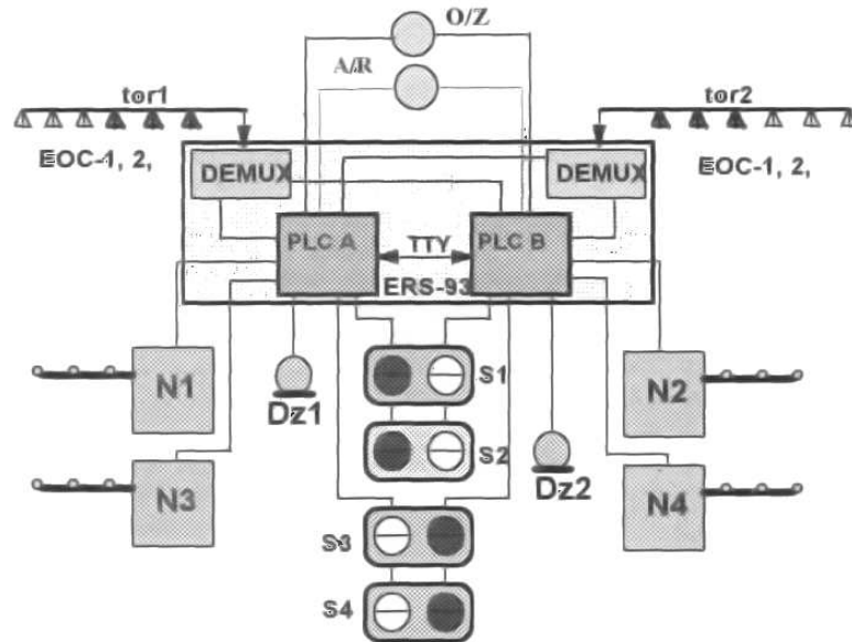
Fig. 2. Redundant structure of the SPA-4 system of level crossing automation
