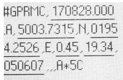
Fig. 6. The SMS screen with the information about the location with the use of the NMEA standard (for the point of measuring no II - Fig. 5)
