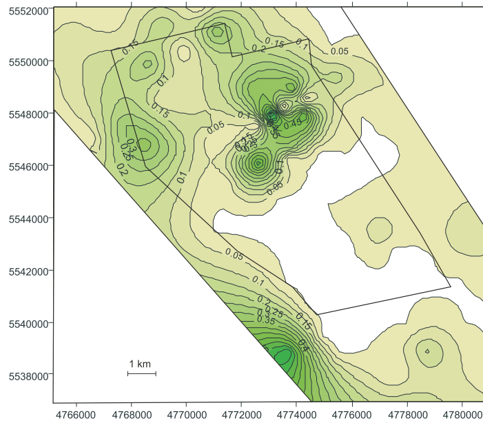
Fig. 4. The thickness of interlayers in the coal seam 382 in the mining area of LW "Bogdanka", LCB
