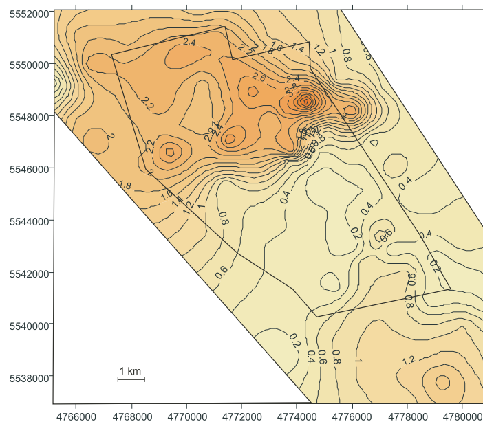
Fig. 3. The thickness of pure coal (without interlayers) in the seam 382 in the mining area of LW "Bogdanka", LCB
