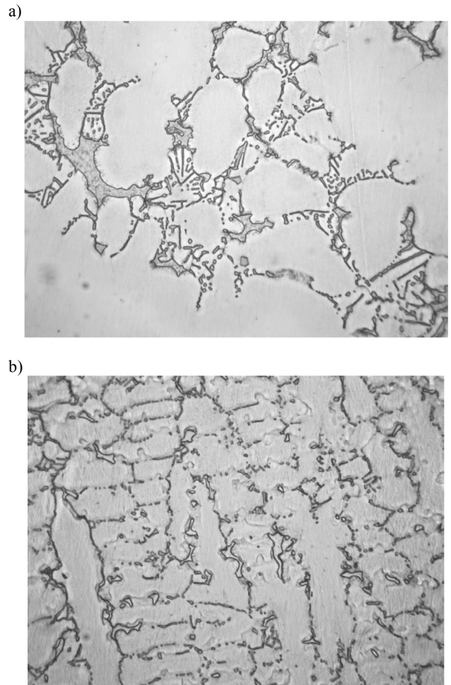
Fig. 2. Microstructure of MAR-M-509 alloy; a) as-cast, b) after rapid resolidification ( I = 200 A, v_s = 250 mm/min)
