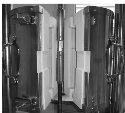
Fig. 4. Stress rupture test stand
