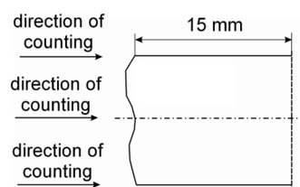
Fig. 6. Designation of the region on metallographic sections and directions for which cracks were counted
