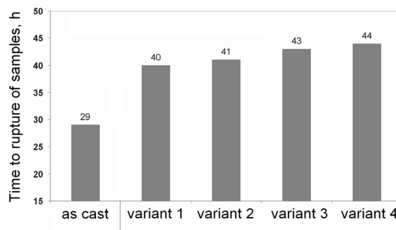
Fig. 5. Time to rupture of MAR-M-509 alloy samples
