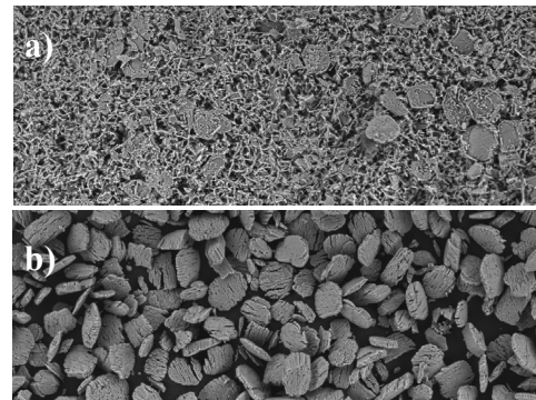
Fig. 3. Images from a Scanning Electron Microscope: a) gypsum GoldStar XL; b) waste gypsum (synthetic); (x250)
