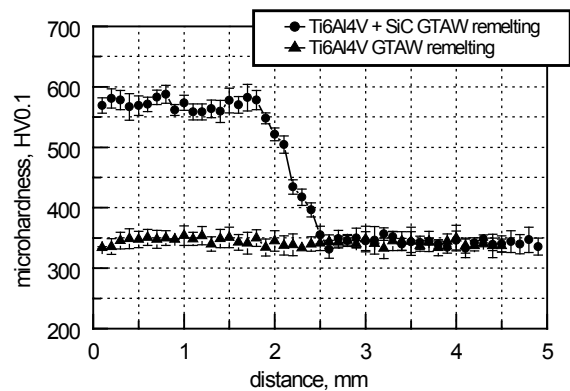
Fig. 10. Microhardness HV0,1 of the Ti6Al4V after remelting and alloying by arc plasma treatment
