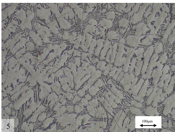
Fig. 3. AISi11 alloy structure: 1 – node; 2 – near node cross-section; 3- cross-section between the nodes; 4- cross-section of closing wall; 5 – outside surface of closing wall
