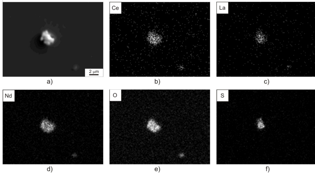
Fig. 5. Oxysulfide type non-metallic inclusion modified with rare earth elements: a – view of the inclusion, (b-f) – distribution maps of elements (steel B after forging)
