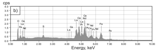
Fig. 4. Oxysulfide type non-metallic inclusion modified with rare earth elements: a – view of the inclusion, b – spectrum of the inclusion (steel B after forging)
