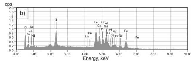
Fig. 3. Oxysulfide type non-metallic inclusion modified with rare earth elements: a – view of the inclusion, b – spectrum of the inclusion (steel A after forging)
