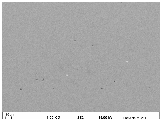
Fig. 2. Very fine non-metallic inclusions on the longitudinal section of the B steel sample
