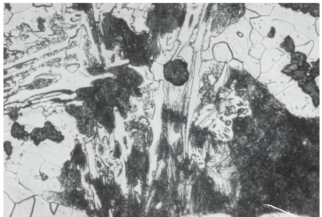
Fig. 4. The microstructure of cast iron from the melt No. 2, etched with Nital, magn. 300×
