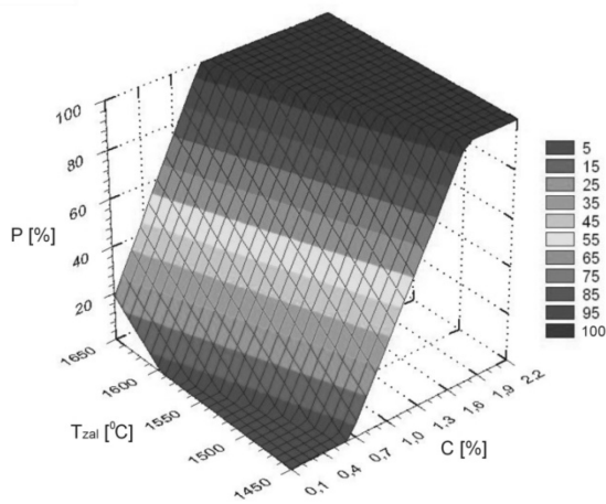
Fig. 4. The influence of pouring temperature and carbon concentration in bearing part on surface on which was obtained permanent joint between the working part (layer) in form of alloy steel X2CrNi 18-9 plate and cast steel in bimetallic layered casting at module 11,45mm
