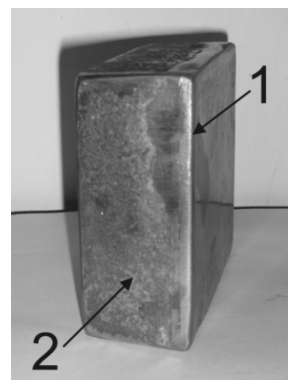
Fig. 6. View of layered casting in configuration: 1 - working part (layer) in form of alloy steel X2CrNi 18-9, 2 - bearing part from unalloyed cast steel at carbon concentration C = 0,96\% and pouring temperature 1650^{\circ}\text{C}
