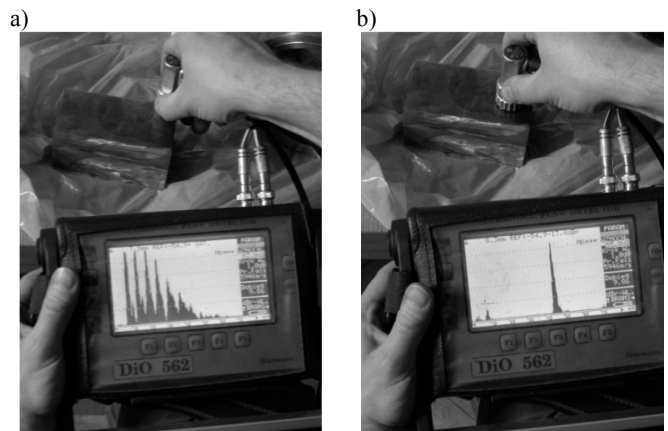
Fig. 2. View of example results of ultrasonic non-destructive testing of bimetallic layered castings: a – lack of joint between the working layer and the bearing part, b – permanent joint between the working layer and the bearing part
