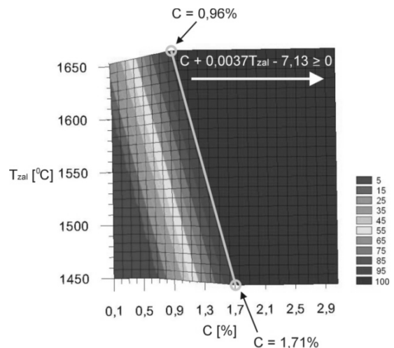
Fig. 5. Graphical interpretation of necessary condition to obtaining the permanent joint on whole contact surface between working part (layer) from alloy steel X2CrNi 18-9 and bearing part from unalloyed cast steel or cast iron in bimetallic layered casting at module 11,45mm
