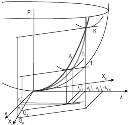
Fig. 1. A paraboloid of the entropy production drawn in function of two thermodynamic forces ( X_c , X_r ), with the added so-called “technological” coordinate system ( v , \lambda ) [5, 6]
