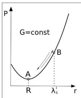
Fig. 2. A parabola of the entropy production for the eutectic rod-like structure formation [5, 6]
